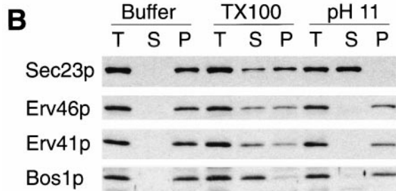
Figure 4. Erv46p and Erv41p are integral membrane proteins. (A) Hydrophilicity plots according to Kyte and Doolittle (1982) with a window size of 7. The schematic representations of the polypeptide chains indicate the positions of the putative transmembrane domains (TM1 and TM2) predicted by the HMMTOP program (Tusnady and Simon, 1998), the region containing conserved cysteine residues (Cys) and the KKXX motif (black dot). (B) Semiintact FY834 cells were treated with buffer (Materials and Methods), buffer containing 1% Triton X-100 (TX100), or 0.1 M Na 2 CO 3 (pH 11) and centrifuged at 100,000 g. Totals before centrifugation (T), supernatant (S), and pellet (P) fractions were analyzed on a 12.5% polyacrylamide gel and immunoblotted for Sec23p (peripheral membrane protein), Erv46p, Erv41p, and Bos1p (integral membrane protein).
