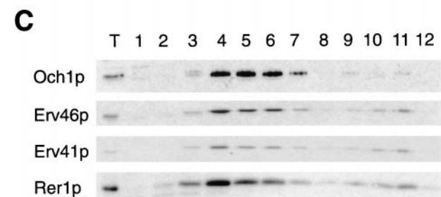
Figure 5. Sucrose gradient fractionation of Erv41p, Erv46p, Och1p, and Rer1p. An FY834 whole cell lysate was separated on an 18–60% sucrose density gradient, and fractions were collected, starting with fraction 1 at the top. (A) Relative levels of Erv41p (Golgi marker), Erv46p (ER marker), and plasma membrane marker (PMA) in each fraction were quantified by densitometry of immunoblots. (B) Relative levels of Och1p, Erv46p, Erv41p, and Rer1p as determined by densitometry of the immunoblots shown in C.
