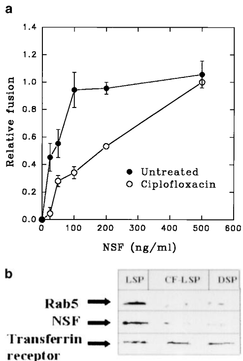
Figure 6. NSF recruitment is dependent on the presence of live Salmonella in phagosome. (a) LSP were prepared as described and treated with ciprofloxacin (500 \mu\text{g/ml} ) at 4^\circ\text{C} for 30 min. NSF on untreated and antibiotic-treated phagosomes were determined as described in Fig. 5 a. Maximum fusion observed in LSP assay was chosen as one unit and the results are expressed as relative fusion of three independent experiments \pm SD. One unit corresponds to \sim 8.92 and 10.3 ng of HRP activity/mg of protein in the fusion assay containing live and dead Salmonella phagosomes, respectively. (b) Determination of rab5 and NSF on different Salmonella -containing phagosome. LSP and DSP were prepared as indicated and bacteria in LSP was killed by ciprofloxacin inside the phagosome (CF-LSP). Phagosomes were washed and the presence of rab5 and NSF on different phagosomes were determined by Western blot analysis using specific antibodies.
