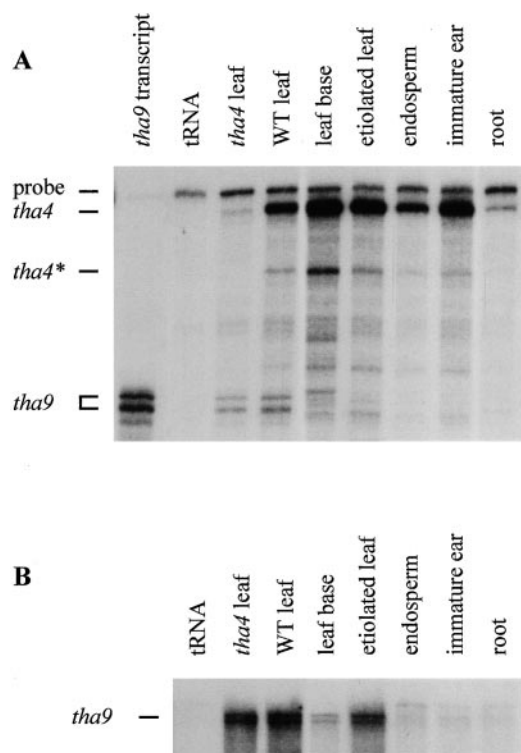
Figure 8. RNase protection analysis of tha4 and tha9 mRNA in different maize tissues. (A) Assays using a tha4 probe. 15 \mu g of total RNA from the indicated maize tissues was analyzed with an antisense probe generated from the tha4 cDNA. Control reactions contained 15 \mu g of tRNA plus 1 \mu g of a sense tha9 transcript generated by in vitro transcription of the tha9 cDNA (first lane) or 15 \mu g of tRNA alone (second lane). The band designated tha4 represents the tha4 mRNA; it is slightly smaller than the full-length probe, which included some vector sequence. The band designated tha4* also results from protection by the tha4 mRNA (note its absence in the tha4 mutant leaf sample); this band may result from a sequence polymorphism between the tha4 probe and tha4 mRNA, resulting in inefficient cleavage of the duplexed probe. The cluster of bands designated tha9 result from protection by the tha9 mRNA. (B) Assays using a tha9 probe. 10 \mu g of total RNA from the indicated maize tissues or 10 \mu g of tRNA (first lane) was analyzed with an antisense probe generated from the tha9 cDNA. The band designated tha9 represents the tha9 mRNA.
