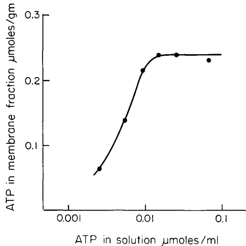
FIGURE 8 ATP binding of membrane fraction as a function of ATP concentration in solution. The solution contained 2.5 mg per ml of membrane fraction. See Methods for further details.
