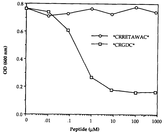
Figure 3. Effect of *CRRETAWAC* and *CRGDC* peptides on binding of RGD-displaying phage to \alpha_5\beta_3 integrin. The cyclic peptides *CRRETAWAC* and *CRGDC* were allowed to compete for the attachment of *CRGDC*-phage to the \alpha_5\beta_3 integrin coated on microtiter wells and phage binding was measured as in Fig. 1. The data show means from duplicate wells.
