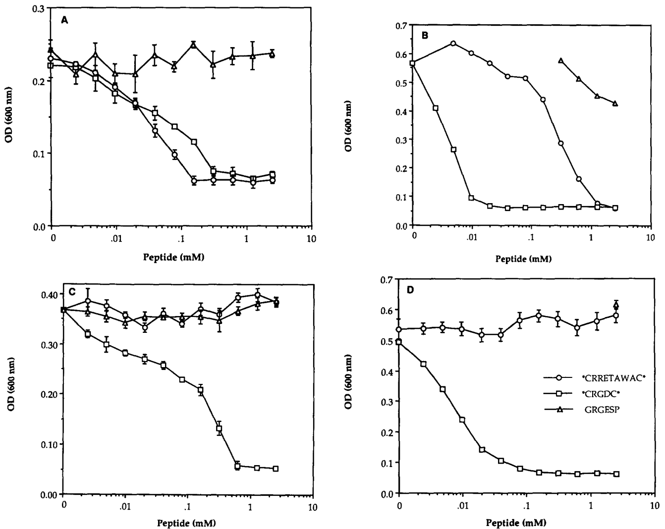
Figure 5. Effect of *CRRETAWAC* peptide on cell attachment to fibronectin and vitronectin. A, B2/α27 cells ( \alpha_5\beta_1 ); B, B2/v7 cells ( \alpha_5\beta_1 ); C, IMR-90 cells ( \alpha_5\beta_3 ); D, HT-29 cells ( \alpha_5\beta_1 ). Cells were allowed to attach for 1 h in microtiter wells coated with fibronectin (A and B) or vitronectin (C and D). The cells that attached were counted as described in Materials and Methods. The data represent means from duplicate wells.
