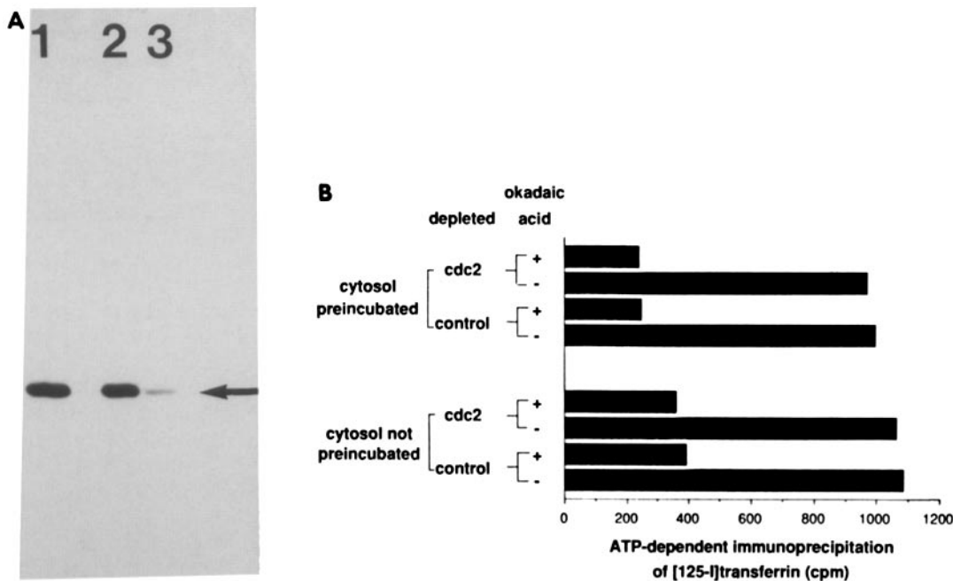
Figure 9. Depletion of cdc2 kinase does not affect inhibition by okadaic acid. (A) 20 \mu g untreated A431 cytosol (lane 1) and cytosol treated with either control (lane 2), or anti-cdc2 (lane 3) protein A-Sepharose beads, were analyzed by Western blotting using a polyclonal antiserum to show the relative concentration of cdc2 kinase protein in each. The position of cdc2 (p34) is indicated by the arrow. (B) Fusion assays were performed using control or anti-cdc2 depleted cytosols in the presence or absence of 1 \mu M okadaic acid. Results are shown from standard incubations, and from incubations where the 30-min preincubation of cytosol was omitted.
