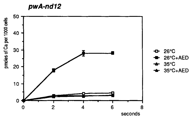
Figure 5. Initial ^{45}\text{Ca} uptake by pwA cells grown at 35°C (a) and by pwA-nd12 (b) grown at 26°C, which is a permissive temperature, and at 35°C which is the nonpermissive temperature. Note that AED provokes a dramatic increase of initial rate of ^{45}\text{Ca} uptake only at 26°C and not at 35°C, although this is possible at that temperature in the absence of the nd12 mutation (a).
