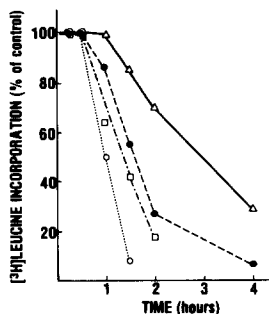
FIGURE 9 Kinetics of inhibition of protein synthesis in CHO pro cells in K + -free medium and normal medium containing NH 4 Cl and nigericin. CHO pro cells were subjected to a 5-min hypotonic shock, then to a 60-min incubation in isotonic \alpha -MEM with or without potassium. The cells were then exposed to 1 \mu g/ml ricin for 10 min. After 10 min, the surface bound ricin was removed by treatment with 0.1 M galactose. After different intervals, the cells were labeled with [ 3 H]leucine for 30 min.
