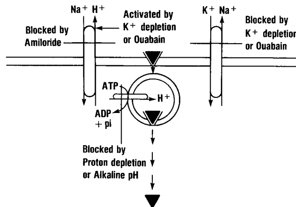
FIGURE 10 Schematic diagram of receptor-mediated endocytosis of ricin and a proposed mechanism for the enhancement of ricin cytotoxicity by K + depletion in CHO cells. \nabla , ricin; V, ricin receptor.
