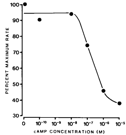
FIGURE 1 The effects of constant concentrations of cAMP on the average rate of motility. 7-h developing cells, at the onset of aggregation, were inoculated into a perfusion chamber and perfused with buffered salts solution containing a single concentration of cAMP. Each point represents the mean for 30 cells. Each cell was monitored for 20 min and the mean rate was calculated. The data is presented as percent maximum rate, which was taken as the average rate of motility in buffered salts solution lacking cAMP. The maximum rate between experiments varied between 9 and 11 \mu\text{m} per minute, but the percent inhibition caused by cAMP between 10^{-7} M and 10^{-5} M was relatively invariant.
