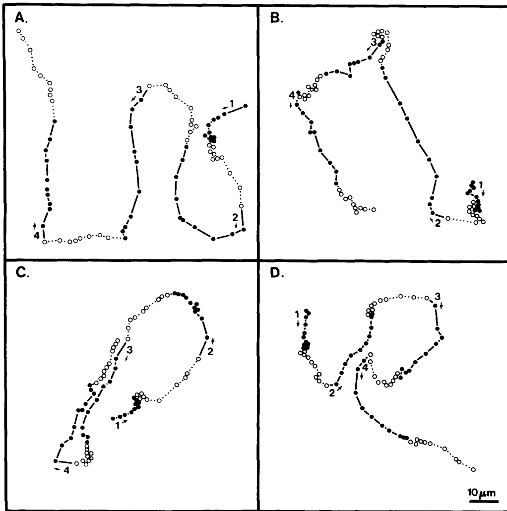
FIGURE 2 The tracks of individual amoebae during four temporal waves of cAMP. The concentration of cAMP during the increasing and decreasing portion of each wave varied between 7.8 \times 10^{-9} to 10^{-6} M as described in the text and diagrammed in the upper portion of Fig. 3. Each panel represents the track of an individual amoeba. The centroid of each individual cell was determined at 21-s intervals during the increasing (●) and decreasing (○) phase of each wave. Consecutive waves are numbered 1 through 4 in each track. The arrows represent the direction of movement.
