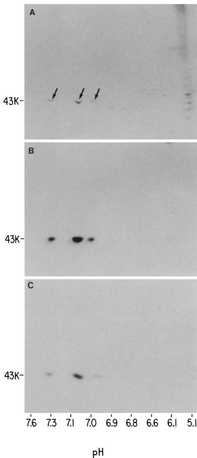
FIGURE 1 Two-dimensional immunoblot analysis of mab specificity. Purified AChR-rich membranes from Torpedo electric organ were subjected to two-dimensional gel electrophoresis. (A) Coomassie Blue-stained gel. Arrows indicate three isoelectric variants of the 43K protein. Identical gels were subjected to immunoblot analysis with (B) mab 1210B or (C) mab 1234A.
