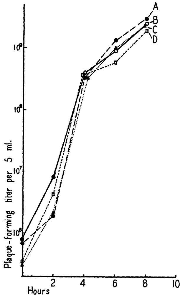
FIG. 5. Growth curves on a monolayer of chicken embryonic cells at different pH of the medium. The pH was controlled by varying the CO 2 tension in the gas atmosphere. The titers refer to the total amount of virus produced in one culture. A, pH 7.8; B, pH 7.4; C, pH 7.2; D, pH 7.0.
