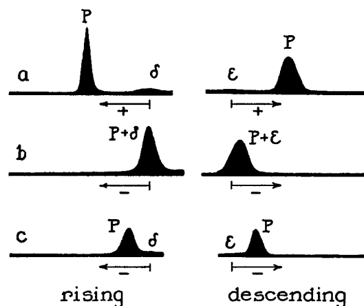
FIG. 2. Precursor, (a) pH 5.0, U_P = 2.72 \times 10^{-5} ; (b) pH 7.3, U_P = -0.074 \times 10^{-5} ; (c) pH 8.6, U_P = -0.94 \times 10^{-5} .
