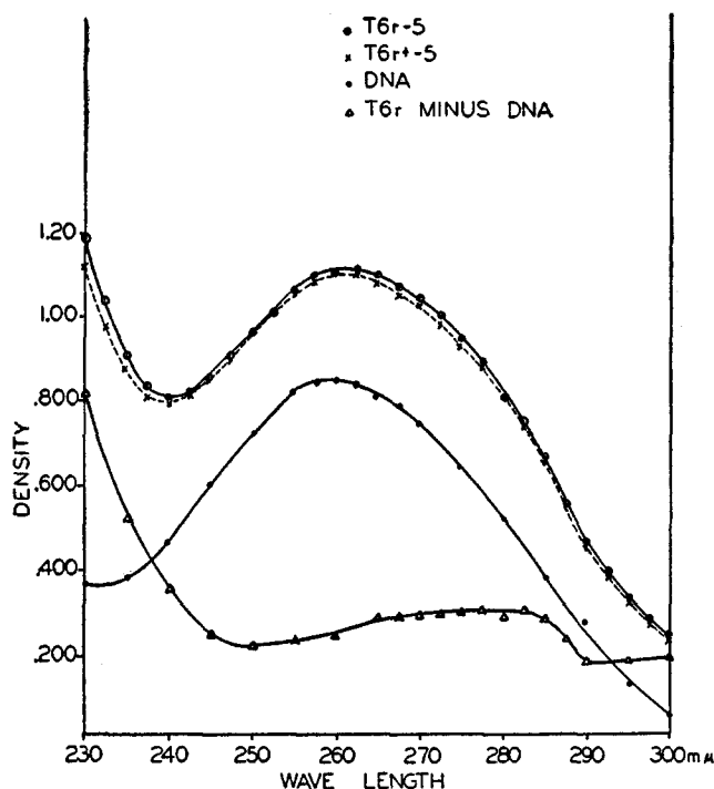
FIG. 2. A comparison of the ultraviolet absorption spectra of T6r + , T6r, and desoxyribose nucleic acid (DNA) at the same DNA concentrations.
