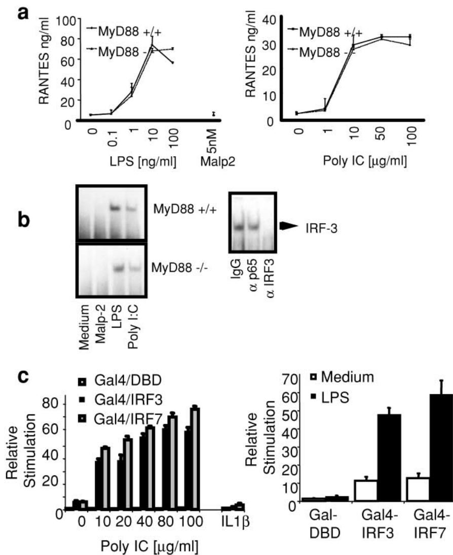
Figure 1. LPS and dsRNA activate IRF-3 and IRF-7. (a) BM-derived macrophages from WT and MyD88-deficient mice were stimulated with LPS (0.1–100 ng/ml), Malp-2 (5 nM), and dsRNA (1–100 \mu\text{g/ml} ) for 12 h. The concentration of RANTES was measured by ELISA. (b) Nuclear extracts were isolated from WT and MyD88-deficient macrophages stimulated with LPS (10 ng/ml), Malp-2 (5 nM), and dsRNA (50 \mu\text{g/ml} ) for 1 h and subjected to EMSA using a ^{32}\text{P} -labeled ISRE consensus sequence (ISG-15) as a probe. Activated complexes were visualized by autoradiography. Activated ISRE DNA-binding complexes were preincubated with polyclonal antibody to IRF-3 or two control antibodies before incubation with the ISRE probe (right). (c) TLR3 and TLR4/MD2-expressing HEK293 cell lines were transfected with a luciferase reporter gene containing the Gal4 upstream activation sequence and with Gal4-DBD , Gal4-IRF-3 , or Gal4-IRF-7 (40 ng). After 24 h, cells were stimulated with LPS (10 ng/ml), dsRNA (50 \mu\text{g} poly IC/ml), IL-1 \beta (10 ng/ml), or left untreated for \sim 8 h, and luciferase reporter gene activity was measured.
