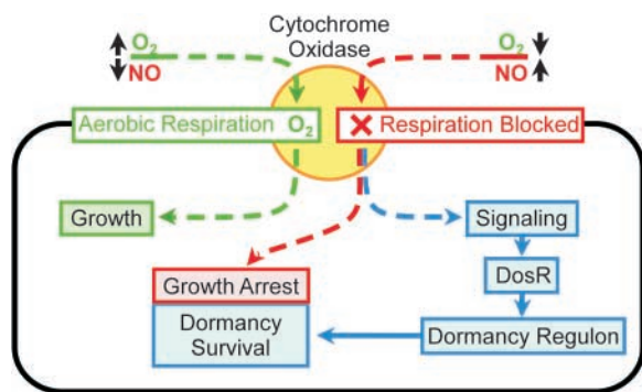
Figure 6. Model of O_2 and NO control of respiration, growth, and gene regulation. Cytochrome oxidase is positioned as the sensor/integrator of O_2 /NO levels in this model.
