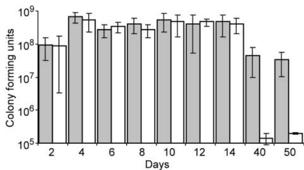
Figure 3. Survival of a dormancy regulon mutant during a low O_2 -induced dormant state. The wild-type H37Rv parent (gray bars) and the Rv3134c mutant (white bars) were grown in the low O_2 -induced dormancy model as described by Wayne and Hayes (11). Bacilli cultures were stirred in sealed test tubes to generate a slow depletion of O_2 via culture respiration. Test tubes were opened to remove samples for colony forming unit determination at each time point and discarded.
