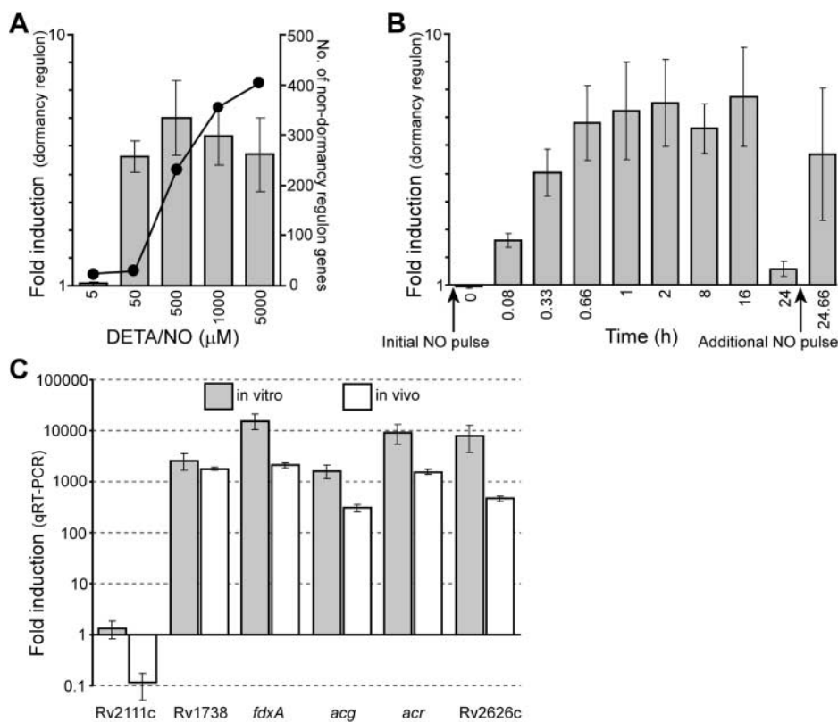
Figure 2. Dormancy regulon gene expression as measured by DNA microarray and qRT-PCR. (A) Average fold induction of all 48 genes as measured by DNA microarray after a 40 min DETA/NO exposure (left y axis); number of nondormancy regulon genes regulated at least twofold (curve; right y axis). (B) Temporal pattern of regulon induction after addition of 500 \mu M DETA/NO. (C) Quantitative in vitro and in vivo (infected mouse lung) induction ratios of the five regulon genes were obtained by qRT-PCR (35). Rv2111c was used as an NO-independent control gene. Gene induction ratios were calculated by first determining the copy number of each transcript normalized to the copy number of the major housekeeping sigma factor gene of M. tuberculosis , sigA . sigA mRNA remained constant during exposure to 50 \mu M DETA/NO (ratio 1:1 as measured by DNA microarray). The normalized copy numbers were compared with mRNA from midlogarithmic phase in vitro grown bacteria. Induction ratios are indicated by gray bars for in vitro exposure to 50 \mu M DETA/NO for 40 min, and white bars indicate in vivo infection, 21 d after challenge.
