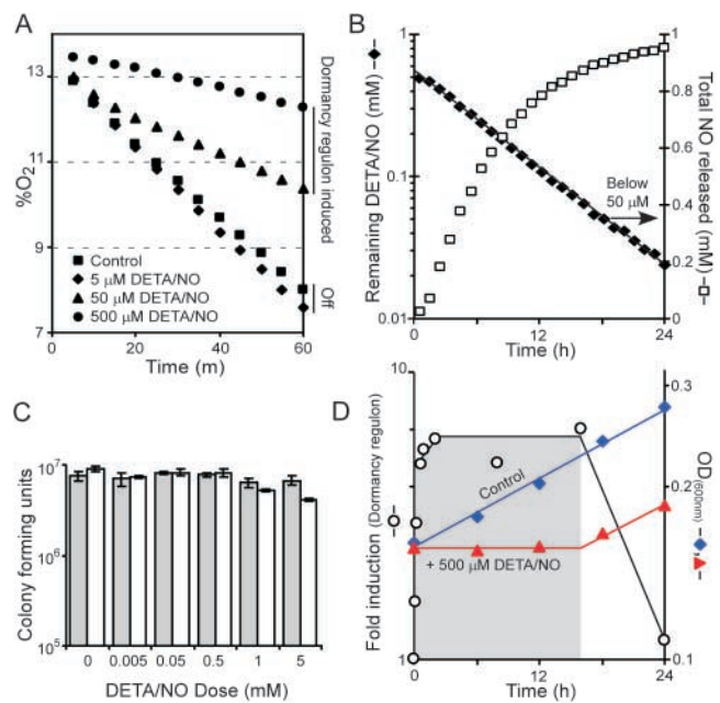
Figure 4. NO-mediated respiratory inhibition and reversible bacteriostasis. (A) The effect of 5, 50, and 500 \mu\text{M} DETA/NO on M. tuberculosis respiration and dormancy regulon induction. DETA/NO was added to a well-aerated 250 ml H37Rv stirring culture and the flask was sealed. A probe measured the depletion of O_2 by bacterial respiration. (B) Rate of DETA/NO decomposition and NO release. DETA/NO release of NO was monitored by absorbance at 252 nm in a 0.1 M phosphate buffer at pH 6.6 and 37°C. A standard curve was generated with known concentrations of DETA/NO to determine the molar absorptivity and used to calculate the DETA/NO concentration (closed diamonds) over time using Beer’s law. One mole of DETA/NO decomposes to release 2 mol NO; therefore, the total NO released (open squares) was calculated by doubling the number of moles of DETA/NO decayed. (C) Survival of M. tuberculosis 1254 monitored by colony-forming units after exposure to various doses of DETA/NO for 4 h (gray bars) and 24 h (white bars). (D) Growth inhibition by NO overlaid with the induction of the dormancy regulon. Average induction of dormancy regulon over time after addition of 500 \mu\text{M} DETA/NO (left y axis); optical density of control culture and culture exposed to 500 \mu\text{M} DETA/NO (right y axis). Refer to Fig. 4 B for the kinetics of NO production and DETA/NO consumption over the same time course after the addition of 500 \mu\text{M} DETA/NO. NO caused a state of bacteriostasis over \sim 16 h. Resumption of growth coincided with the disappearance of NO as indicated by reduction of regulon expression to basal levels (gray area) and decomposition of the NO donor (B).
