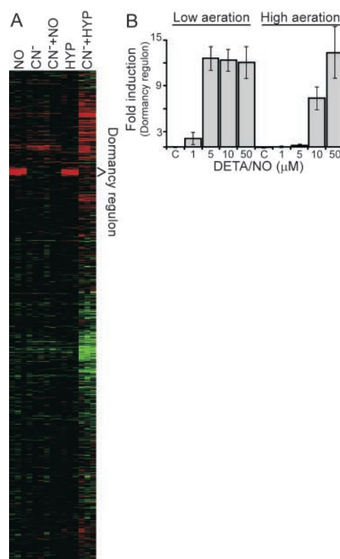
Figure 5. Competition between O_2 and NO for heme-containing protein. (A) Average linkage clustering comparison of expression data from all M. tuberculosis genes after a 40-min exposure to 50 \mu\text{M} DETA/NO, 50 \mu\text{M} KCN, KCN plus DETA/NO, 2-h hypoxia, and 500 \mu\text{M} KCN plus 2-h hypoxia. (B) Competition between NO and O_2 for control of dormancy regulon expression. DETA/NO was added to a 300-ml culture stirring at 100 rpm for low aeration and maximum rpm for high aeration. Induction of the regulon was assayed by DNA microarray after 40 min NO exposure.
