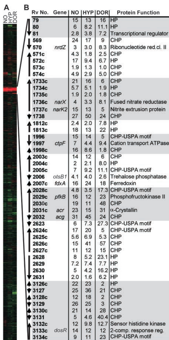
Figure 1. Dormancy regulon. Comparison of microarray expression results from M. tuberculosis strain 1254 exposed for 40 min to 50 \mu M of the NO donor DETA/NO (NO), and strain H37Rv exposed for 2 h to 0.2% O 2 (hypoxia-HYP) and at day 4 during the gradual adaptation, to low O 2 as described previously (11), resulting in an in vitro dormant state (DOR). DNA microarrays were used for the NO and low O 2 experiments, whereas oligonucleotide microarrays were used for the DOR experiments. (A) All M. tuberculosis genes are represented and organized based on their regulatory profile by average linkage clustering, using the Cluster and Treeview programs. Red indicates induced, green indicates repressed, and black indicates no change in gene expression. (B) The initial selection of genes in the dormancy regulon was based on their coinduction by NO, low O 2 , and adaptation to an in vitro dormant state, as well as their failure to be induced in the presence of KCN (see Fig. 3 A). Rv numbers designate genes in genomic order, and arrows indicate transcript direction. Annotations are from TubercuList ( http://genolist.pasteur.fr/TubercuList ; reference 34). CHP and HP indicate conserved hypothetical and hypothetical proteins.
