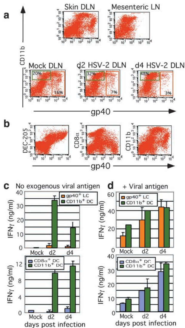
Figure 7. Submucosal DCs, but not Langerhans cells or CD8 \alpha^{+} DCs, present viral peptides to CD4 ^{+} T cells in the draining lymph nodes. To differentiate the contribution of LCs and submucosal DCs in the presentation of HSV-2 antigens in vivo , CD11c ^{+} cells were stained with gp40 (LC) and CD11b (submucosal DC) after HSV-2 ivag infection at 2 or 4 d a.i. and were analyzed by flow cytometry (a). The DC markers, DEC-205, CD8 \alpha , and CD11b, on CD11c ^{+} cells were analyzed (b). The LC-derived (gp40 ^{+} ), submucosal DCs (CD11b ^{+} ), or the CD8 \alpha^{+} DCs were FACS ^{\text{R}} -sorted from draining lymph nodes at 2 or 4 d a.i. and were co-cultured with HSV-2-specific CD4 ^{+} T cells in the absence (c) or presence (d) of viral antigens for 72 h. IFN \gamma secreted from T cells were analyzed by ELISA (c and d).
