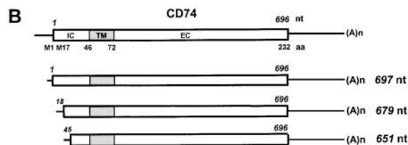
Figure 3. Identification by expression cloning of CD74 as a cell surface binding protein for MIF. (A) Progressive enrichment by fluorescence-activated cell sorting of COS-7 cell transfectants showing MIF binding activity. (B) Structure of CD74 (35-kD isoform), and 3 of 10 representative CD74 cDNA clones with MIF binding activity. IC, TM, and EC are the intracellular, transmembrane, and extracellular domains, respectively. M1 and M17 refer to two sites of alternative translation initiation (42).
