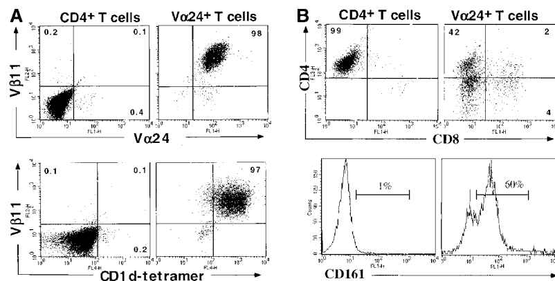
Figure 1. Phenotype of in vitro -expanded NKT cells. Purified CD4 + T cells were activated by SEB (100 ng/ml) and purified V \alpha 24 + T cells were stimulated with \alpha -GalCer (100 ng/ml) in the presence of autologous DCs. Cells were expanded in IL-2 for 14 d. (A) To determine expansion of NKT cells in vitro -expanded T cell lines were stained with anti-V \beta 11-PE, anti-V \alpha 24-FITC, and CD1d-tetramer-APC. (B) Expression of CD4, CD8, and NK markers on SEB-stimulated CD4 + or \alpha -GalCer-stimulated NKT cell lines. Cells were costained with anti-CD4-PerCP and anti-CD8-FITC, and individually stained with purified anti-CD161 followed by FITC-conjugated anti-mouse IgG.
