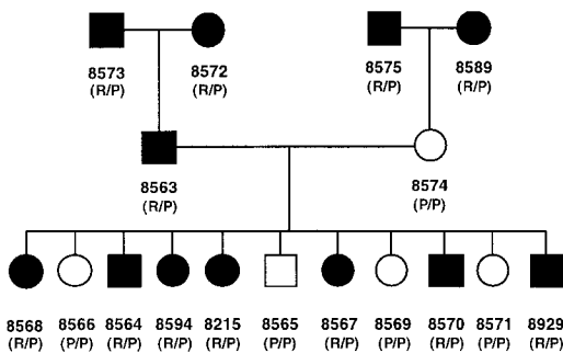
Figure 5. HA-8 mHAg allelic segregation analysis. Segregation of the HA-8 R and HA-8 P alleles and correlation of the HA-8 R allele with cytolysis by SKH-13 CTLs at an E/T ratio of 5:1 is shown using the BLCL of CEPH reference family 1362. Filled circles (females) or squares (males) indicate strong lysis by SKH-13 CTLs (phenotype positive); open symbols indicate minimal lysis (phenotype negative). Numbers below symbols were assigned to each family member by the University of Utah. R/P represents HA-8 R/P heterozygous genotype; P/P represents HA-8 P genotype (the HA-8 P/liter polymorphism cannot be distinguished by these genotyping PCR primers). Genotyping of HA-8 mHAg alleles was determined by PCR-RFLP of genomic DNA as described in Materials and Methods.
