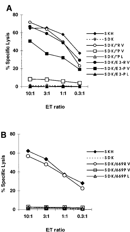
Figure 7. Comparative SKH-13 CTL recognition of transiently transfected KIAA0020 constructs. (A) CTL recognition of the donor-derived BLCL SDK is shown after transient transfection of experimental minigene constructs. Constructs tested contain a minigene cassette encoding the KIAA0020 polymorphic peptides either with (closed symbols) or without (open symbols) an E3-19K adenovirus leader peptide sequence, which directs translocation of the expressed peptide to the ER, bypassing normal TAP transport. CTL lysis of donor (SDK) and recipient (SKH) BLCL is also shown. (B) Eukaryotic expression plasmids expressing a truncated KIAA0020 protein initiating from the native start codon, encoding RTLDKVLEV, PTLDKVLEV, or PTLDKVLEL without an E3-19K adenovirus leader peptide sequence, were transiently transfected into SDK BLCL as described in Materials and Methods and incubated with the SKH-13 CTL clone in a standard epitope reconstitution assay. CTL lysis of recipient (SKH) and donor (SDK) BLCL cells is indicated.
