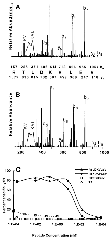
Figure 2. Identification of the HA-8 mHAg antigenic peptide. (A) CAD mass spectrum of candidate peptide ( M+2H ) ^{2+} ion with monoisotopic m/z of 536.834 ^{+2} as eluted from JY BLCL. (B) CAD mass spectrum of synthetic peptide RTLDKVLEV. Mass spectra were recorded on a Finnigan LCQ ion trap MS operating with a 3.0 atomic mass unit isolation window and 35% collision energy. The b and y ions (reference 54) are labeled above and below the amino acid sequence, respectively. Ions observed in the spectrum are underlined. (C) HA-8 mHAg epitope reconstitution with synthetic peptides. A standard ^{51}\text{Cr} -release assay was performed by incubating the indicated quantities of synthetic peptides with ^{51}\text{Cr} -labeled T2 target cells and then adding the mHAg-specific CTL clone SKH-13. An E/T ratio of 10:1 was used. FIDSYICQV corresponds to the mHAg A2-HY (reference 25), and serves as a negative control. Background lysis of T2 by the CTLs in the absence of any peptides was 4%; positive control lysis was 87%.
