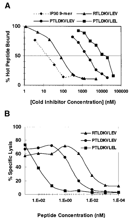
Figure 6. HLA-A*0201 binding affinity of HA-8 mHAg peptide variants and SKH-13 CTL recognition of exogenously pulsed peptide variants. (A) Binding of RTLDKVLEV, PTLDKVLEV, and PTLDKVLEL to HLA-A*0201. HPLC-purified synthetic peptides were assayed for their ability to inhibit the binding of the iodinated peptide FLPSDYFPSV (◆) to affinity-purified HLA-A*0201 molecules in a cell-free peptide binding assay (see Materials and Methods). (B) RTLDKVLEV, PTLDKVLEV, and PTLDKVLEL were tested for their ability to reconstitute the epitope for the SKH-13 CTL clone. Epitope reconstitution assay conditions are described in Materials and Methods. An E/T ratio of 10:1 was used. Background CTL lysis of T2 in the absence of any peptides was 4%; positive control lysis (SKH) was 80%.
