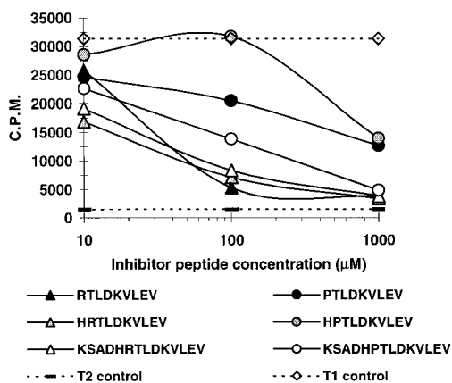
Figure 8. In vitro transport of HA-8 mHAg peptide variants. T1 cells were permeabilized with streptolysin O (15 U/ml) and incubated with radioiodinated reporter peptide TVNKTERAY plus the indicated dilution of test peptides. Reporter peptide transport in TAP-negative T2 cells was assessed as a negative control. Samples were done in duplicate except for T2 negative control and T1 cells with no inhibitor, which were done in triplicate.
