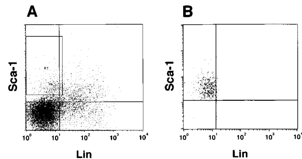
Figure 1. Isolation of Sca1 + lin -dim hematopoietic progenitors from fetal liver cells. Pooled day 13.5 gestation fetal liver cells from each respective genotype were prepared for culture by isolation of low density cells using a Ficoll-Hypaque gradient. Low density cells were simultaneously stained with isotype controls or antibodies to Sca1 (PE) and lineage markers including anti-B220 (pan-B lymphocytes), anti-CD3 \epsilon (pan-T cells), anti-Gr-1 (granulocytes), and anti-Mac 1 (monocyte-macrophages) all conjugated to FITC. Sca1 + lin -dim cells were identified relative to isotype control antibodies in the upper left corner of the dual parameter dot plot in A. These cells were isolated by fluorescence-activated cell sorting and a sample of sorted cells was reanalyzed to confirm the purity of isolated cells (B).
