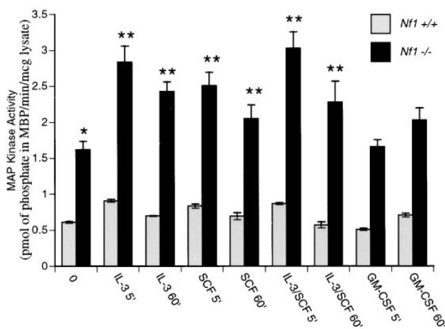
Figure 5. MAP kinase activity in c-kit + hematopoietic cells. c-kit + bone marrow cells from mice previously reconstituted with Nfl^{-/-} or Nfl^{+/+} fetal liver cells were isolated, stimulated with cytokines for specified times, and harvested, and cell lysates were prepared. MAP kinase activity was measured in whole cell extracts. Activity was calculated by determining the rate of incorporation of phosphate in MBP per min/ \mu g of lysate and is indicated in the graph for each genotype, cytokine, and length of stimulation. The genotype and length of stimulation are indicated.
