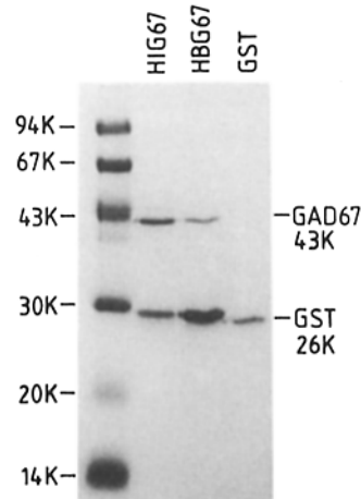
Figure 1. SDS-PAGE analysis of glutathione affinity purified recombinant GST fusion proteins. Proteins were subjected to electrophoresis in a 12.5% acrylamide gel and stained with coomassie blue. Lane 1, molecular size markers; lane 2, GST-human islet GAD67; lane 3, GST-human brain GAD67; lane 4, GST.
