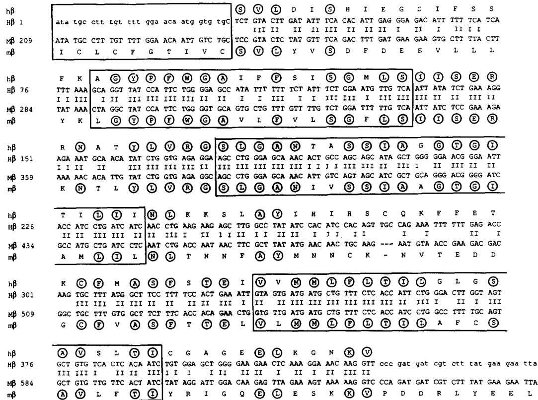
Figure 4. Analysis of the human basophil cDNA fragment amplified with murine Fc \epsilon RI \beta -derived oligonucleotides. Nucleotide sequence of the human cDNA fragment (H \beta ) is compared with the murine Fc \epsilon RI \beta cDNA (M \beta ). Conserved bases are linked by (I). The numbers in the left margin refer to the nucleotide position within the human cDNA fragment or the published murine cDNA sequence (14). Sequences of the primers are noted in small letters. The deduced amino acid sequence encoded by the human cDNA is given using the single-letter code (h \beta ), and is compared with the murine Fc \epsilon RI \beta amino acid sequence (m \beta ); (circles) conserved residues. (Boxes) transmembrane domains (14). Note that the intracytoplasmic domain (IISER . . . . YLVRG) is well conserved in human and mouse.
