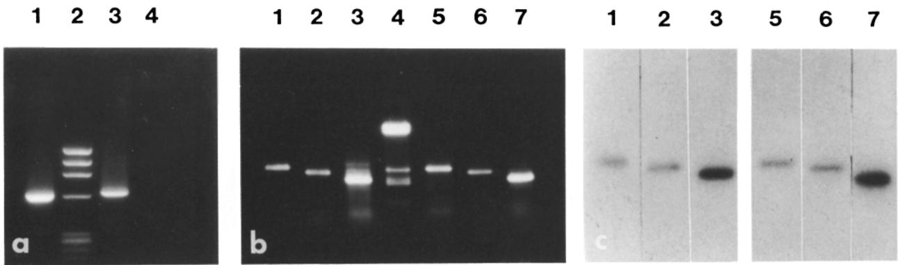
Figure 3. Analysis of RT-PCR-amplified transcripts of tryptase ( a ) and of the \alpha , \beta , and \gamma subunits of Fc \epsilon RI ( b and c ) from human purified LC ( a , lane 4; b and c , lanes 1-3), from human basophils ( a , lane 1; b and c , lanes 5-7), and the cell line KU812 ( a , lane 3). Purified LC were prepared by immunomagnetic separation, and basophils were obtained by gradient density centrifugation of peripheral blood. ( a and b ) Ethidium bromide staining of the electrophoretic gels. ( c ) Autoradiogram of the Southern blot hybridized with oligonucleotides specific for the three subunits of Fc \epsilon RI. Fc \epsilon RI \alpha : b and c , lanes 1 and 5. Fc \epsilon RI \beta : b and c , lanes 3 and 7. Fc \epsilon RI \gamma : b and c , lanes 3 and 7. Sizes of HaeIII-digested \phi \chi 174 (1,358, 1,078, 872, 603, and 310-bp DNA fragments): a , lane 2, and of Taq 1-digested pBR322 (1,444, 1,305, 475, 368, 315, 313, and 141-bp DNA fragments): b , lane 4.
