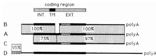
Figure 2. A diagram of the regions of homology in the DNA sequences of the NKG2 transcripts. The shaded areas refer to the percent homology between the adjacent transcripts. The stippled region within the NKG2-A, -B, and -C transcripts is 95% homologous with the 5' end of NKG2-D. Heavy bars indicate the protein coding regions.
