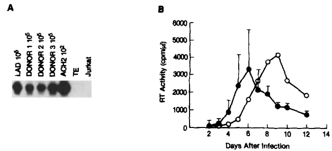
Figure 1. (A) Oligomer hybridization of amplified HIV-1 (LAV) DNA from in vitro infected PHA-activated LFA-1 - and LFA-1 + cells. Intensity of the PCR signals in 10^5 LFA-1 - cells and 10^5 LFA-1 + cells from three different donors are compared (TE, buffer control; DNA lysates from 10^5 Jurkat, negative control; DNA lysates from 10^2 ACH2, a cell line containing a single proviral copy of HIV per cell [12], positive control). The results shown were obtained using gag primer pairs and probe. Similar results were obtained with LTR primer pairs and probe. (B) Comparative analysis of the levels of virus replication in LFA-1 - and LFA-1 + cell cultures. Levels of virus replication in LFA-1 - (O) and LFA-1 + (●) cells infected with HIV-1. LFA-1 - and LFA-1 + PBMC were stimulated for 72 h with PHA and inoculated with SNs containing HIV-1 LAV . The levels of RT activity observed in HIV-infected LFA-1 - cell cultures are representative of three independent experiments and are compared with levels of RT activity (mean \pm SD) in HIV-infected LFA-1 + cell cultures from six normal donors.
