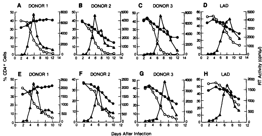
Figure 3. Involvement of the LFA-1 molecule in HIV-mediated depletion of CD4 + T lymphocytes. In A-C and E-G , PHA-activated LFA-1 + cells infected with HIV-1 and HIV-2, respectively, were obtained from three normal donors. In D and H , PHA-activated LFA-1 - cells were infected with HIV-1 and HIV-2, respectively. ( \blacktriangle ) Levels of RT activity; ( \bullet ) percentage of CD4 + cells in uninfected cultures; ( \circ ) percentage of CD4 + cells in cell cultures infected either with HIV-1 or HIV-2. Infection of PHA-activated LFA-1 - and LFA-1 + cells with HIV-1 and HIV-2 and the staining of CD4 + cells were performed as described in Materials and Methods.
