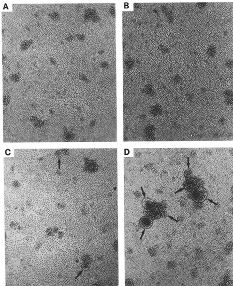
Figure 2. Role of the LFA-1 molecule in cell fusion and syncytia formation. Small clumps, but not syncytia, were observed in uninfected ( A ) and in HIV-1 ( B ) or HIV-2 (data not shown) -infected LFA-1 - cell cultures. In contrast, syncytia formation ( arrows ) occurred in LFA-1 + cell cultures infected with HIV-1 ( C ), and to a greater extent in those infected with HIV-2 ( D ). Photomicrographs ( \times 75 ) were taken at day 5 after infection in the experiments in B-D . Cultures were scored daily for syncytia formation. Infection of PHA-activated LFA-1 - and LFA-1 + cells with HIV-1 and HIV-2 were performed as described in Materials and Methods.
