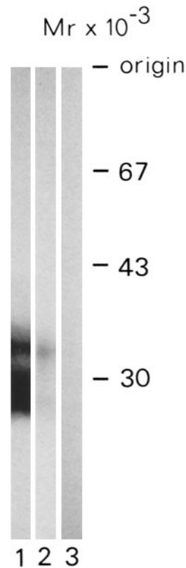
FIGURE 7. EA 1 synthesis by T cells activated with TPA is inhibited by cycloheximide. TPA activated T cells were labeled with [ ^{35}\text{S} ]methionine in the absence of cycloheximide (lane 1) and in the presence of 50 \mu\text{M} cycloheximide (lane 2) and 500 \mu\text{M} cycloheximide (lane 3).
