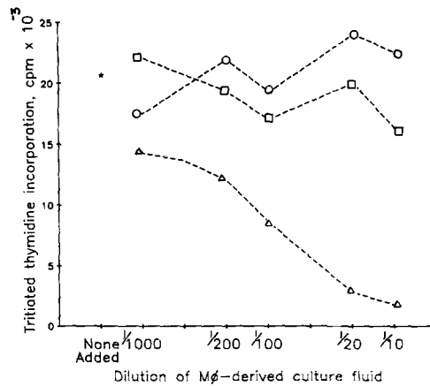
FIGURE 2. IL-1 inhibitor activity produced in 24 h by control macrophages (○) and macrophages exposed to influenza virus (□) or RSV (△). ★, thymocyte proliferation in the presence of purified IL-1 in the absence of macrophage fluids.
