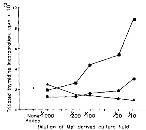
FIGURE 1. IL-1 activity produced in 24 h by control macrophages (Mφ) (●) and macrophages exposed to influenza virus (■) or RSV (▲). ★, thymocyte proliferation in the absence of macrophage fluids.
