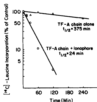
FIGURE 1. Kinetics for inhibition of cellular protein synthesis by TF-A chain. Receptor sites were saturated by treating K562 cells with 10^{-7} M TF-A chain for 10 min and then transferrin was added at 10^{-5} M to block toxin interaction with recycled receptor. The cells were then incubated for designated intervals at 37^{\circ}\text{C} in leucine-free media alone ( \Delta ) or with 10^{-7} M monensin ( \circ ) before pulsing with [ ^{14}\text{C} ]leucine (30 min) and assaying incorporation. When excess transferrin was added before TF-A chain exposure, levels of incorporation were comparable to untreated cells and this served as a control for each time point.
