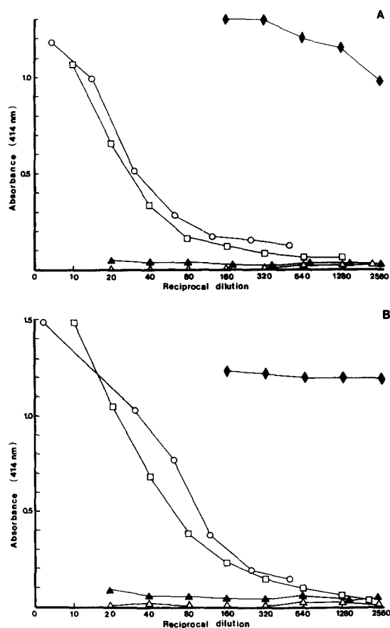
FIGURE 1. Binding by ELISA of MAb directed against idiotypic determinants of the TEPC-15 immunoglobulin to limulin and CRP. MAb tested: 4C11 (A) and F6 (B). Proteins: TEPC-15 (◆), CRP (□), limulin (○), D. candidum lectin (▲), and BSA (△).
