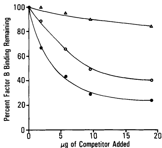
FIG. 4. Acquisition of affinity for Factor B by methylamine treatment of C3. Competition by fluid-phase C3 ( \Delta ), C3(CH 3 NH 2 ) (O), and C3b (●) with the binding of 125 I-Factor B to E s C3b. The assays contained 5 \times 10^7 E s C3b and 2 \mu g 125 I-Factor B in a final volume of 100 \mu l DGVB that contained 4 mM MgCl 2 . Binding was determined after 10 min at 21°C by measuring the decrease of radioactivity in the fluid phase after removal of the cells.
