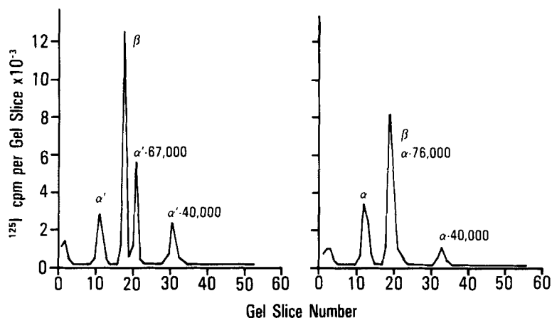
FIG. 5. Cleavage of C3(CH 3 NH 2 ) by C3bINA and \beta 1H. (Left) Polyacrylamide gel electrophoresis in the presence of SDS and dithiothreitol of 125 I-C3b after a brief incubation with C3bINA and \beta 1H. The two \alpha' -chain cleavage products, \alpha' -67,000 and \alpha' -40,000, are indicated. (Right) Similar treatment of 125 I-C3(CH 3 NH 2 ) showed only the \alpha' -40,000 and a proportional increase in radioactivity in the 75,000 M r \beta -chain peak. The \alpha -76,000 chain appears to be composed of \alpha' -67,000 and covalently linked C3a.
