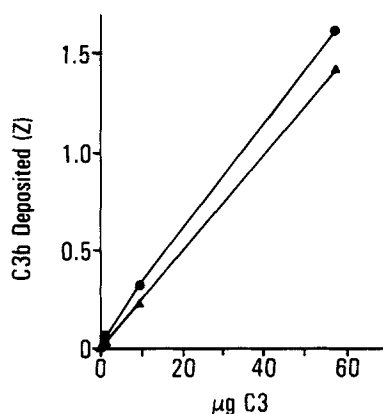
FIG. 8. Deposition of C3b on sheep erythrocytes ( E_s ) by a fluid-phase C3 convertase containing C3(CH 3 NH 2 ). Fluid-phase conversion of various amounts of native C3 to C3b in the presence of E_s was catalyzed by properdin(P)-stabilized C3 convertases that contained either C3(CH 3 NH 2 ) or C3b. Deposited C3b was assayed as described in Materials and Methods. ●, C3b, Bb, P; ▲, C3(CH 3 NH 2 ), Bb, P.
