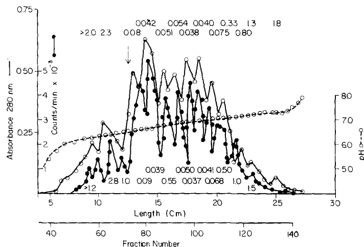
FIG. 7. Comparison of IEF profiles obtained with polyacrylamide gel (250 \mu g of protein, open circles) or with Sephadex G-75 Superfine (55 mg of protein, filled circles) as supporting medium. The protein is specifically purified anti-Ar antibody from mouse 23. The numbers shown in the graph indicate the weight of protein in the corresponding peak required to cause 50% inhibition of binding in the standard assay system (same system as in Fig. 1). The upper set of numbers refers to the upper curve (open circles); the lower set to the lower curve (filled circles). The length plotted on the abscissa refers to the distance measured along the length of the Sephadex slab; the fraction numbers refer to the polyacrylamide gel. The pH range in each case was 5-8. The arrow indicates the position of application of the sample in the Sephadex gel.
