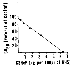
FIG. 8. Quantitative relation between the amount of isolated C3NeF added to NHS and the resultant reduction in hemolytic activity. 6.4 \mu\text{g} of C3NeF caused 100% loss of the activity of 100 \mu\text{l} serum.
