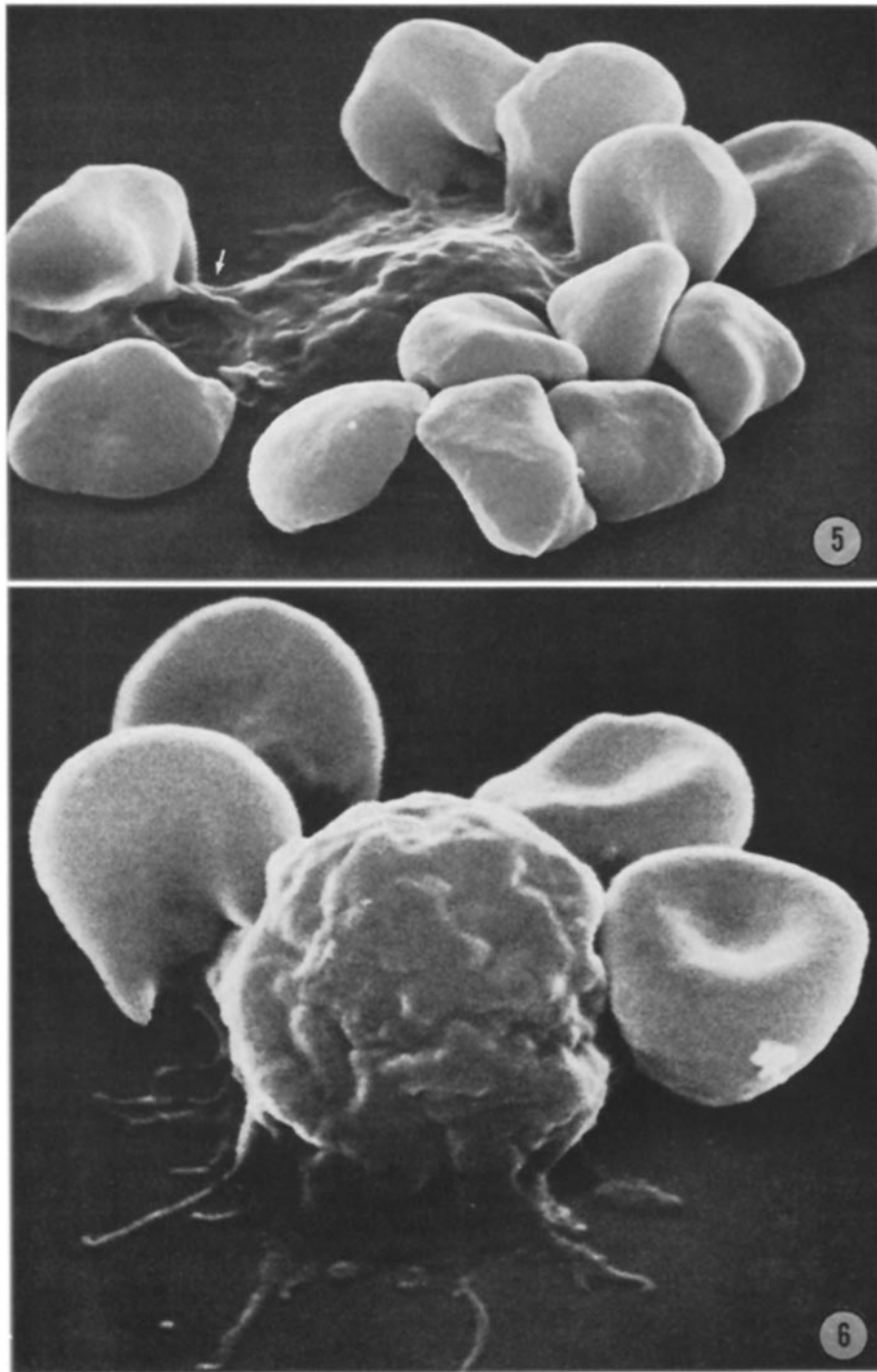
FIG. 5. Large RFC with spotlike contacts between cytoplasmic folds and red cells (arrow). Fixed at 330 mosM. \times 6,500.
