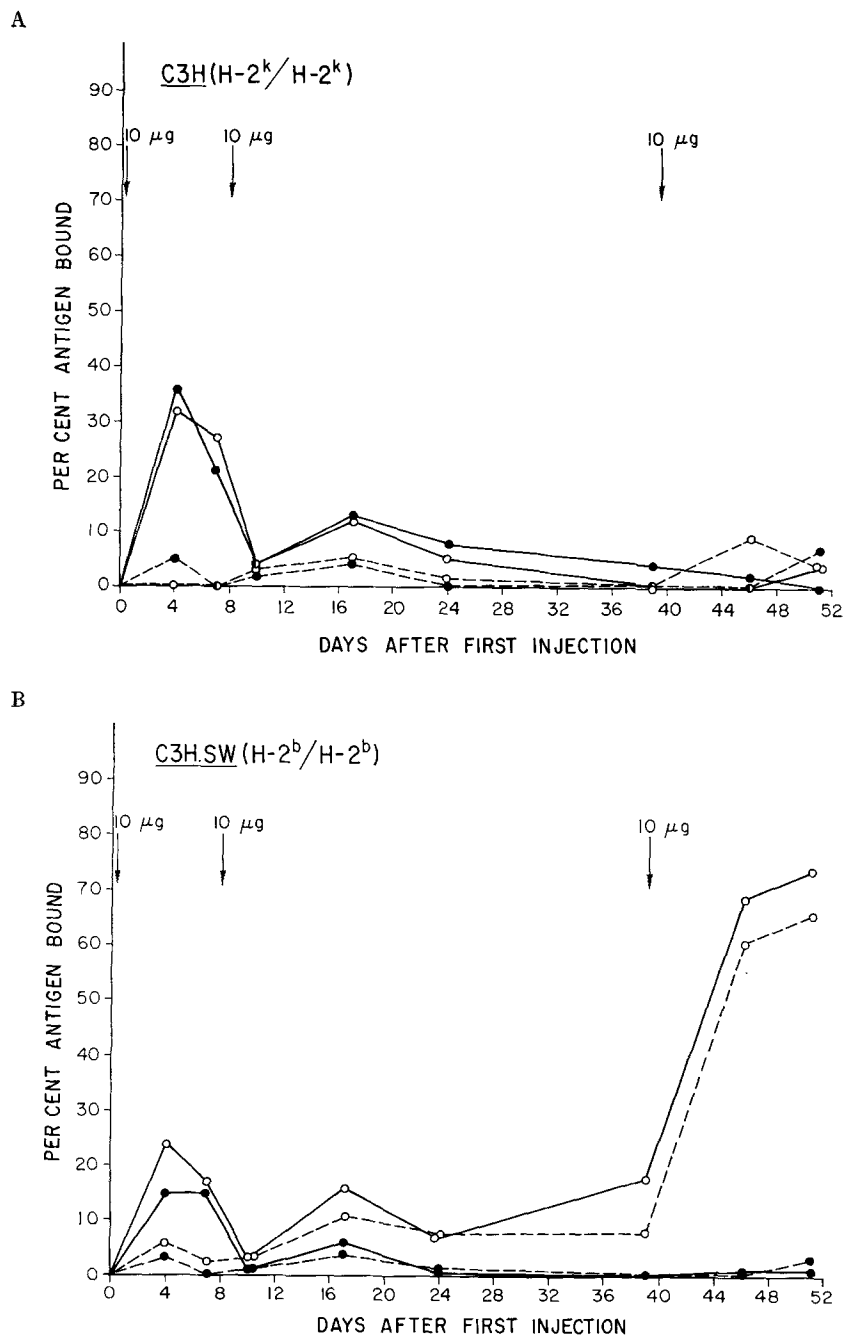
FIG. 1. The response of adult thymectomized or sham-thymectomized mice to 10 \mu g of aqueous (T,G)-A-L given intraperitoneally on days 0, 8, and 39: (a) C3H mice; (b) C3H.SW mice. Sham-thymectomized total antibody, —○—; sham-thymectomized 2-Me-resistant antibody, ---○---; thymectomized total antibody, —●—; thymectomized 2-Me-resistant antibody, ---●---.
