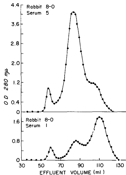
FIG. 5. Gel filtration on Sephadex G-200 of serum 1 and 5 of rabbit 8-0. Column dimensions, 40 \times 2 cm. Protein concentration in the fractions was determined by measuring absorbency at 280 m \mu .
