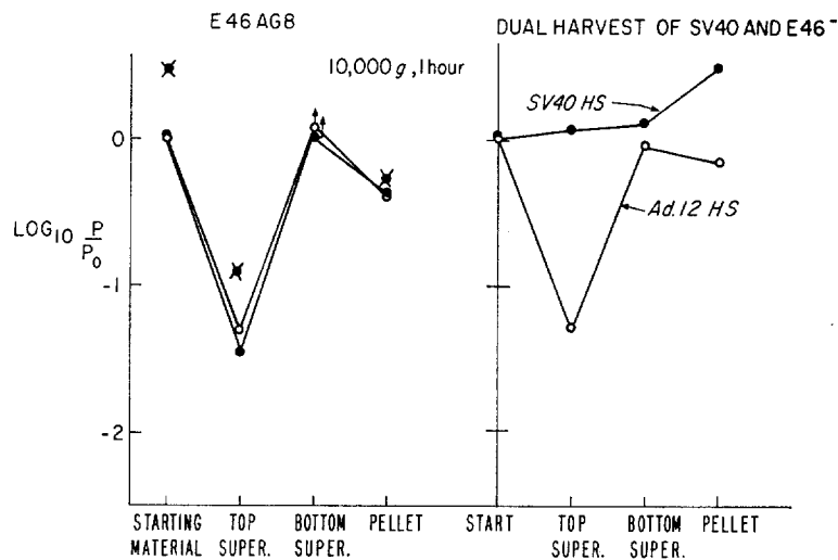
FIG. 5. Ultracentrifugation of E46 + and Ad. 7-SV40 mixed infection preparations, assayed by first cycle neoantigen induction. \times indicates SV40 neoantigen staining of fractions assayed with E46 - helper. HS, tumored hamster serum. The passage level beyond the E46 pool is identified by "AG" followed by the number of passages.
