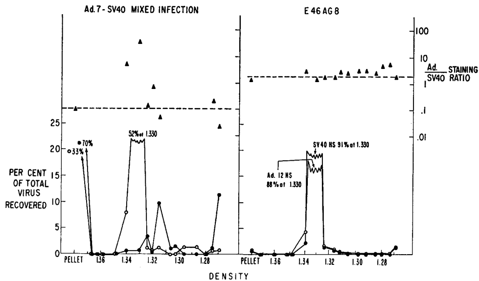
FIG. 4. Equilibrium density gradient centrifugation of E46 + and Ad. 7-SV40 mixed infection preparations, assayed by first cycle neoantigen induction. O, Ad. 12-tumored hamster serum; ●, SV40-tumored hamster serum; ▲, Staining ratio. The dashed line is the staining ratio of the starting material. The passage level beyond the E46 pool is identified by "AG" followed by the number of passages.
