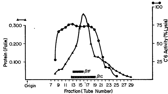
TEXT-FIG. 2. Electrophoretic separation of non-activated (untreated) TEAE fraction of rabbit serum, pH 8.6. A wide zone of C'6 activity is present with smaller central zones of C'5 ( \beta 1F) and \beta 1C-globulin. See text for details.
