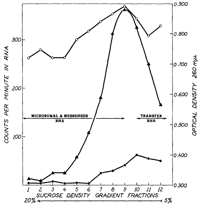
FIG. 4. Effect of actinomycin D on synthesis of various fractions of RNA separated in sucrose density gradient: O, total RNA as measured spectrophotometrically at 260 mμ, ▲, CPM in RNA of non-inhibited control cells; ●, CPM in RNA of cells exposed to 1 μg/ml of actinomycin D.
