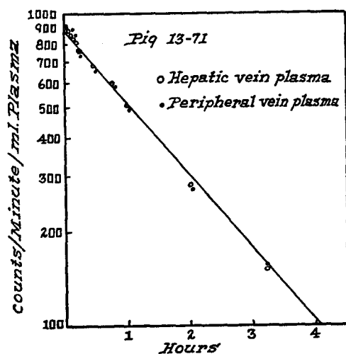
FIG. 3. Disappearance of \text{Fe}^{59} from plasma obtained simultaneously from hepatic and peripheral vein.
