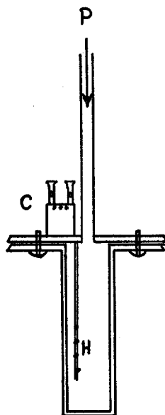
FIG. 1. Diagram of the chamber containing the water or red cells and the thermopile. H , the warm junctions, C the cold reference junctions, and P the tube through which the pressure is suddenly applied.
