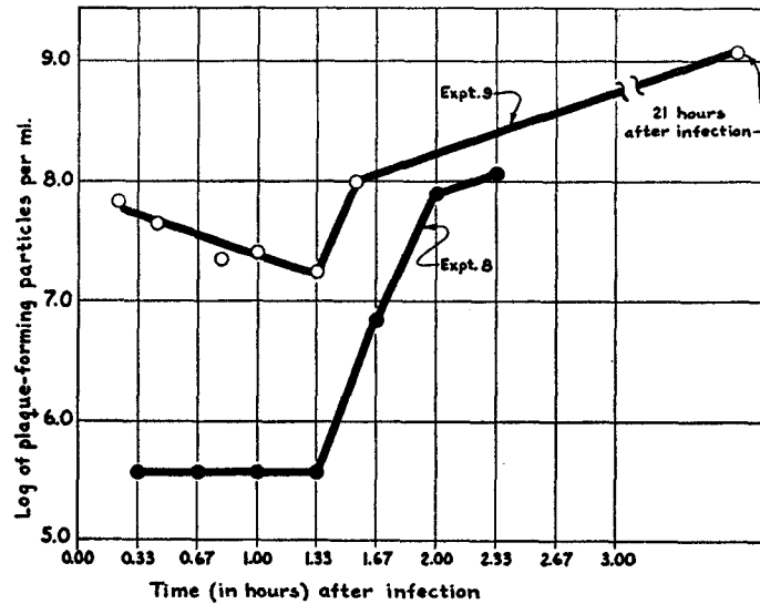
FIG. 15. Experiments B8 and B9. Phage multiplication in suspensions of cells containing 10^6 and 10^7 cells per ml. respectively.
