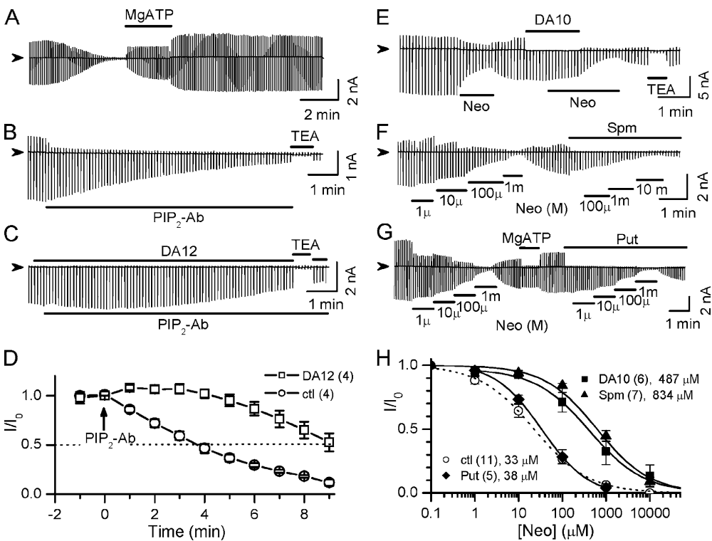
Figure 3. Long polyamines strengthen the PIP 2 -channel interaction in wild-type Kir2.1 channels. (A) Channel activity shows minimal rundown after reactivated by treatment with 2 mM MgATP. (B) After exposure to 2 mM MgATP to minimize spontaneous rundown, application of PIP 2 antibody (PIP 2 -Ab) induced rundown with a half-time of ~4 min. (C) DA12 (100 μM) slowed PIP 2 -Ab-induced rundown. (D) Average time course of rundown induced by PIP 2 -Ab under control (ctl) and in the presence of DA12 (100 μM). Currents (I) are normalized to the value before PIP 2 was added (I 0 ). (E) Ramp pulse-elicited current traces showing differential inhibitory effect of 100 μM neomycin (Neo) in the absence and presence of 100 μM DA10. (F) Neomycin sensitivities in the absence and presence of 100 μM spermine. (G) Neomycin
