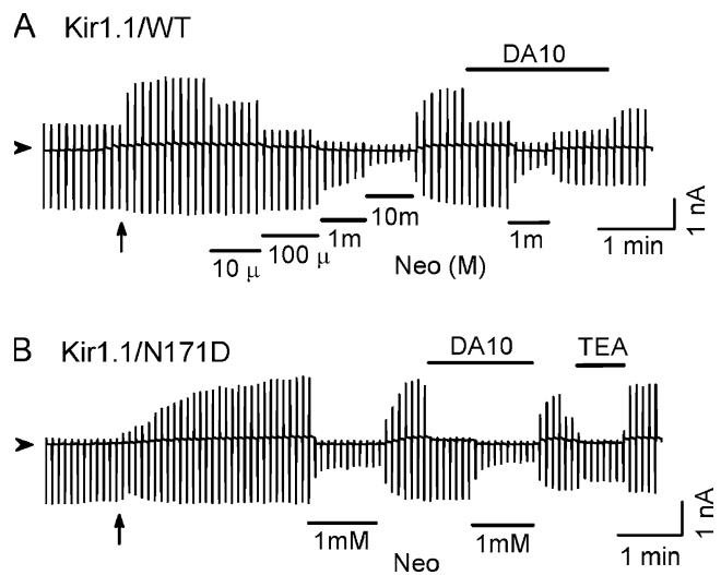
Figure 6. Long polyamines do not strengthen the \text{PIP}_2 –channel interaction in Kir1.1 channels. (A) Ramp pulse–elicited current traces were recorded from wild-type Kir1.1 channels. DA10 (100 \mu\text{M} ) did not cause any shift in neomycin (Neo) sensitivity. Note the same degree of inhibition by 1 mM neomycin in the absence or presence of 100 \mu\text{M} DA10. (B) Same as A, except for Kir1.1/N171D mutant channels. The extent of inward rectification was enhanced in this mutation. However, DA10 (100 \mu\text{M} ) had no effect on neomycin sensitivity. TEA (30 mM) had less effect on the inward currents.
