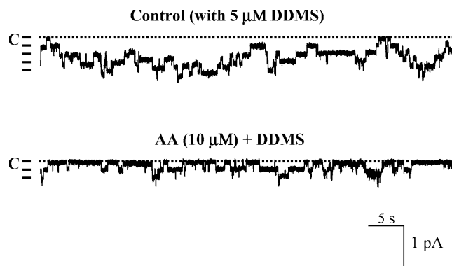
FIGURE 6. A channel recording showing the effect of 10 \mu\text{M} AA on ENaC in the presence DDMS. The channel closed level is indicated by a dotted line.
