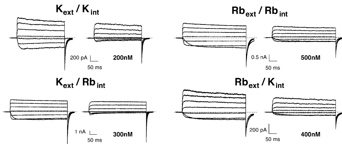
FIGURE 2. \kappa -PVIIA block of Shaker currents in symmetric and asymmetric ionic Rb^+ or K^+ solutions. Current records in response to IV protocols ( V_H = -100 mV, V_p from -50 mV to +70 mV, every 20 mV) recorded with outside-out patch clamp experiments in symmetrical 115 mM KCl (top left), symmetrical 115 mM RbCl (top right), K_{ext}/Rb_{int} (bottom left), and Rb_{ext}/K_{int} (bottom right) before and after the addition to the bath of \kappa -PVIIA (concentration indicated in the figure). The reversal potential is +5 mV in symmetrical 115 mM KCl, +3 mV in symmetrical 115 mM RbCl, +4 mV in K_{ext}/Rb_{int} , and -5 mV in Rb_{ext}/K_{int} .
