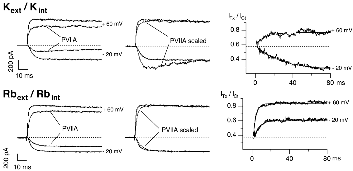
FIGURE 1. \kappa -PVIIA blocks Shaker currents differently in symmetrical K^+ and Rb^+ . (Left) Current responses to voltage steps from a holding potential of -100 mV to -20 and +60 mV, under control conditions and with 200 nM \kappa -PVIIA in symmetrical K^+ (top) and 500 nM \kappa -PVIIA in symmetrical Rb^+ (bottom). (Middle) Current in toxin is scaled to the control to evidence the effect of the toxin. Note that besides a reduction in the current amplitude, also a modification in the kinetics of the current is observed. (Right) Ratio between the toxin and control current traces. The dotted lines correspond to the tonic unblock for closed state, respectively 0.58 in K^+ and 0.37 in Rb^+ , corresponding to a K^O of 265 nM and 293 nM, respectively. The single exponential fits are superimposed to the traces: in symmetrical K^+ (top) at +60 mV, \tau = 9.56 ms and U = 0.76 ; at -20 mV, \tau = 27.2 ms and U = 0.26 . In symmetrical Rb^+ (bottom) at +60 mV, \tau = 4.6 ms and U = 0.87 ; at -20 mV, \tau = 5.65 ms and U = 0.60 .
