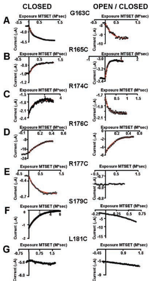
FIGURE 9. Time course of MTSET modification. Currents were measured at the end of the test pulse. Monoexponential fits are superimposed (red lines). (A) Time course of MTSET modification of the G163C mutant. (B) Time course of MTSET modification of the R165C mutant. (C) Time course of MTSET modification of the R174C mutant. (D) Time course of MTSET modification of the R176C mutant. (E) Time course of MTSET modification of the R177C mutant. Notice that in this case only closed channels are modified by MTSET. (F) Time course of MTSET modification of the S179C mutant. Only closed channels are modified by MTSET. (G) Mutant L181C was insensitive to the MTSET treatment in both closed and open/closed states.
