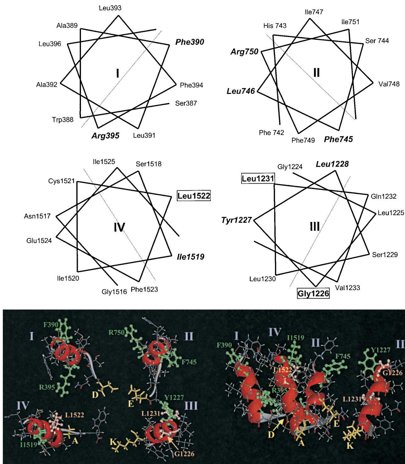
FIGURE 6. Structure of Na channel SS1 region of the P segments. (top) Helical wheel representations of the residues mutated in this study. The residues in bold italics are accessible from the aqueous pore; those enclosed in a box do not express current and thus have an indeterminate phenotype. The cysteine mutants that alter \text{Cd}^{2+} /TTX block sensitivity or have an indeterminate phenotype are on the same side of the helix. (bottom) Molecular model of the putative pore helices in the Na channel pore, views from the top (left) and side (right) are shown. The domains are positioned to approximate the distances between selectivity filter residues. The pore helices are rendered in ribbon format, the DEKA ring in yellow stick format, and accessible (green) or nonfunctional (salmon) positions in ball-and-stick format.
