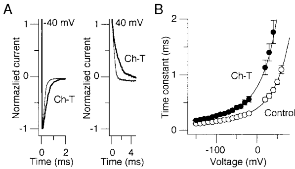
FIGURE 5. Deactivation is slowed by Ch-T. (A) Representative tail currents recorded at -40 mV (left) and 40 mV (right) after 15 -ms pulses to 220 mV before and after Ch-T treatment ( 2 mM for 1 min). In each panel, the tail current recorded after Ch-T treatment (thick sweep) is slower. The results shown were obtained without any added Mg^{2+} . (B) Voltage dependence of deactivation. Tail currents recorded at different voltages were fitted with a single exponential excluding the initial 100 \mu s. The time constant values estimated before (open circles) and after (closed circles) Ch-T treatment ( 2 mM, 1 min) are plotted as a function of voltage. At every voltage examined, the time constant value was greater after Ch-T treatment. Voltage dependence of the time constant ( \tau(V) ) was fitted by the equation \tau_A(0) \cdot \exp(z_A FV/RT) + \tau_B(0) \cdot \exp(z_B FV/RT) , where \tau_A(0) and \tau_B(0) are the time constant values of the two components at 0 mV, z_A and z_B are their respective equivalent charges, F is Faraday's constant, R is the gas constant, and T is temperature. The values of \tau_A(0) and \tau_B(0) in the control condition were 0.14 \pm 0.1 ms and 0.25 \pm 0.1 ms. Their respective values after Ch-T treatment were 0.44 \pm 0.2 ms and 0.61 \pm 0.5 ms. The values of z_A and z_B before Ch-T treatment were 0.12 \pm 0.05e and 0.77 \pm 0.26e . After Ch-T treatment, their values were 0.16 \pm 0.13e and 0.74 \pm 0.30e ( n = 10 ). The correlation coefficient ( r ) values between \tau_A(0) and the current amplitude at 240 mV ( I_{240} ), \tau_B(0) and I_{240} , z_A and I_{240} , and z_B and I_{240} in the control condition were 0.082 , -0.41 , 0.27 , and 0.13 , respectively.
