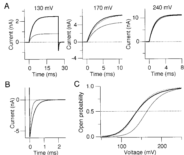
FIGURE 14. Simulation of the Ch-T effects using the HCA model. (A) Ionic currents simulated by the HCA model at 130, 170, and 240 mV. The control hSlo currents recorded without any added Mg^{2+} were simulated using the model of Horrigan et al. (1999) with the following parameter values: \alpha(0) = 1,500 s ^{-1} , \beta(0) = 35,370 s ^{-1} , \delta_0(0) = 0.007 s ^{-1} , \delta_1(0) = 0.154 s ^{-1} , \delta_2(0) = 3.39 s ^{-1} , \delta_3(0) = 52 s ^{-1} , \delta_4(0) = 65 s ^{-1} , D = 22 , f = D^{0.5} , L(0) = \delta_0(0)/\gamma_0(0) = 2 \times 10^{-6} . The equivalent charge values are as in Horrigan et al. (1999) and they are as follows: z_\alpha = 0.275e , z_\beta = -0.275e , z_\delta = 0.262e , and z_\gamma = -0.138e . Each of the simulated channels ( n = 200 ) has a linear conductance value of 250 pS and the reversal potential was set at 0 mV. To simulate the effects of Ch-T, the following parameter values were used: \alpha(0) = 3,500 s ^{-1} , \delta_0(0) = 0.003 s ^{-1} , \delta_1(0) = 0.066 s ^{-1} , \delta_2(0) = 1.45 s ^{-1} , \delta_3(0) = 52 s ^{-1} , \delta_4(0) = 65 s ^{-1} . In each comparison, the thin data sweep represents the control data sweep and the thick data sweep represents the data after simulated Ch-T. At 170 mV, the simulated control current was scaled up to compare the activation kinetics (dashed line). (B) Simulated tail currents at -150 mV before (thin sweep) and after (thick sweep) simulated Ch-T application. The currents were simulated as in A. (C) Open probability curves as a function of voltage before (thin curve) and after (thick curve) simulated Ch-T application. The data were simulated as in A. The dotted line represents the simulated control curve shifted along the voltage axis to match the simulated Ch-T data.
