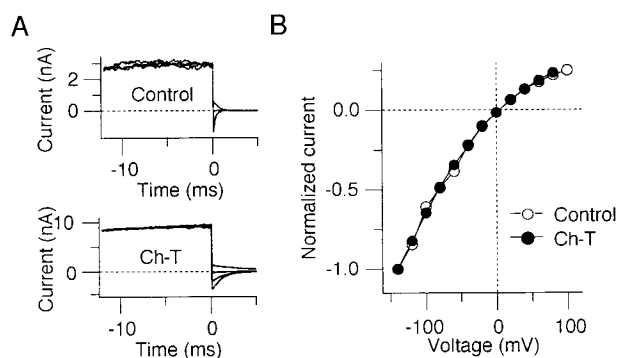
FIGURE 4. Ch-T does not modify instantaneous tail I-V. (A) Representative tail currents recorded at -40 , -20 , 0 , and 20 mV before (top) and after (bottom) Ch-T application ( 5 mM for 1 min). The currents were elicited by 30 -ms pulses from -70 to 130 mV. In the experiment shown, Ch-T increased the current at 130 mV by \sim 200\% . The results shown were obtained without any added Mg^{2+} . (B) Scaled instantaneous tail I-V curves obtained before (open circles) and after (closed circles) Ch-T application ( 5 mM for 1 min). The tail currents were fitted by a single exponential and the instantaneous ( t = 0 ) currents were estimated by extrapolation. The current amplitudes at different voltages were scaled to the extrapolated tail current amplitudes at -150 mV.
