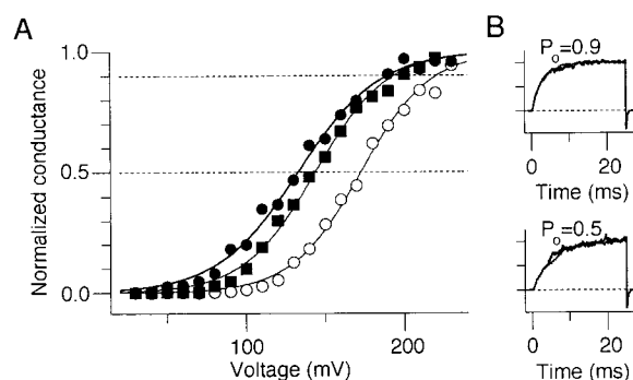
FIGURE 8. V_{0.5} shift induced by Ch-T is mimicked by 300 nM Ca^{2+} . (A) Macroscopic hSlo G-V curves were recorded in 0.2 nM [Ca^{2+}] (11 mM EGTA, no added Ca^{2+} ; open circles), 300 nM [Ca^{2+}] (11 mM EGTA, 7 mM Ca^{2+} ; squares), and then in 0.2 nM [Ca^{2+}] after Ch-T treatment (2 mM for 1 min; closed circles). The currents were elicited by pulses to different voltages and the tail currents were recorded at -45 mV. The V_{0.5} values for the above conditions were 173, 144, and 133 mV, respectively; the Q_{app} values were 1.15, 1.1, and 0.97, respectively. The results shown were obtained without any added Mg^{2+} . (B) Scaled macroscopic currents recorded at the voltages where the open probability values were 0.9 (top) and 0.5 (bottom). In each comparison, the currents recorded in 300 nM [Ca^{2+}] (thin sweep) and in 0.2 nM [Ca^{2+}] after Ch-T treatment (thick sweep) are shown. For the comparison at P_o = 0.9 , the currents recorded at 190 mV in the two conditions are scaled and shown. For the comparison at P_o = 0.5 , the current in 300 nM [Ca^{2+}] at 140 mV and the current in 0.2 nM [Ca^{2+}] after Ch-T at 130 mV are scaled and shown.
