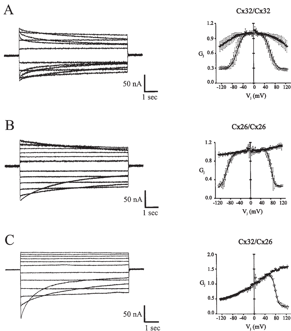
Figure 1. Conductance–voltage relations and representative traces of initial and steady state junctional currents obtained in pairs of Xenopus oocytes. (A) Cx32 homotypic junctions. (B) Cx26 homotypic junctions. (C) Cx32/Cx26 heterotypic junctions. Initial conductance is depicted by \blacktriangledown , and steady-state conductance by \nabla . In all cases, positive V_j is relative positivity at the cytoplasmic mouth of the hemichannel appearing on the right side of the channel designation. For example, in the heterotypic junction, the x axis gives the V_j of the Cx26 side of the junction. The conductance–voltage relations of each junction are the average of at least 10 separate oocyte pairs.
