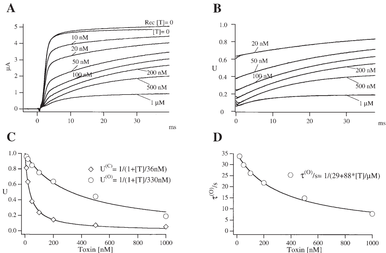
Figure 3. Dose response of PVIIA effects on ShA channels. (A) Voltage-clamp currents for a voltage step to +20 mV from a holding potential of −100 mV recorded from the same oocyte exposed at increasing values of [T] as indicated. The trace marked “Rec[T] = 0” was recorded after washing out the 1 μM PVIIA solution; notice a small “run up” and a residual slow unblock indicating that a few nanomolar PVIIA are still present around the oocyte. (B) Ratios, U, of the toxin to the initial control responses in A are plotted vs. dt = (t - t_{1/2}) , where t_{1/2} is the time of half activation of the control response; single-exponential fits (smooth lines) are indistinguishable from the data for dt > 1 ms; departures at earlier times are likely due to inadequate voltage-step control. (C) [T] dependence of the extrapolated values of the U(t) data in B for dt = 0 ( U^{(C)} ) and dt \rightarrow \infty ( U^{(O)} ); the solid lines are best fits with Langmuir isotherms: U = 1/(1 + [T]/K) . The fitted K values for U^{(C)} and U^{(O)} data are, respectively, K^{(C)} = 36 nM and K^{(O)} = 330 nM. (D) [T] dependence of the time constant \tau^{(O)} of the exponential fits in B; the solid line is the best fit with the expression: \tau^{(O)} = 1/(k_{off}^{(O)} + k_{on}^{(O)} [T]) ; the fitted parameters are k_{off}^{(O)} = 29 s −1 and k_{on}^{(O)} = 88 μM −1 s −1 ; the ratio k_{off}^{(O)}/k_{on}^{(O)} coincides with K^{(O)} = 330 nM from the fit of U^{(O)} data in C.
