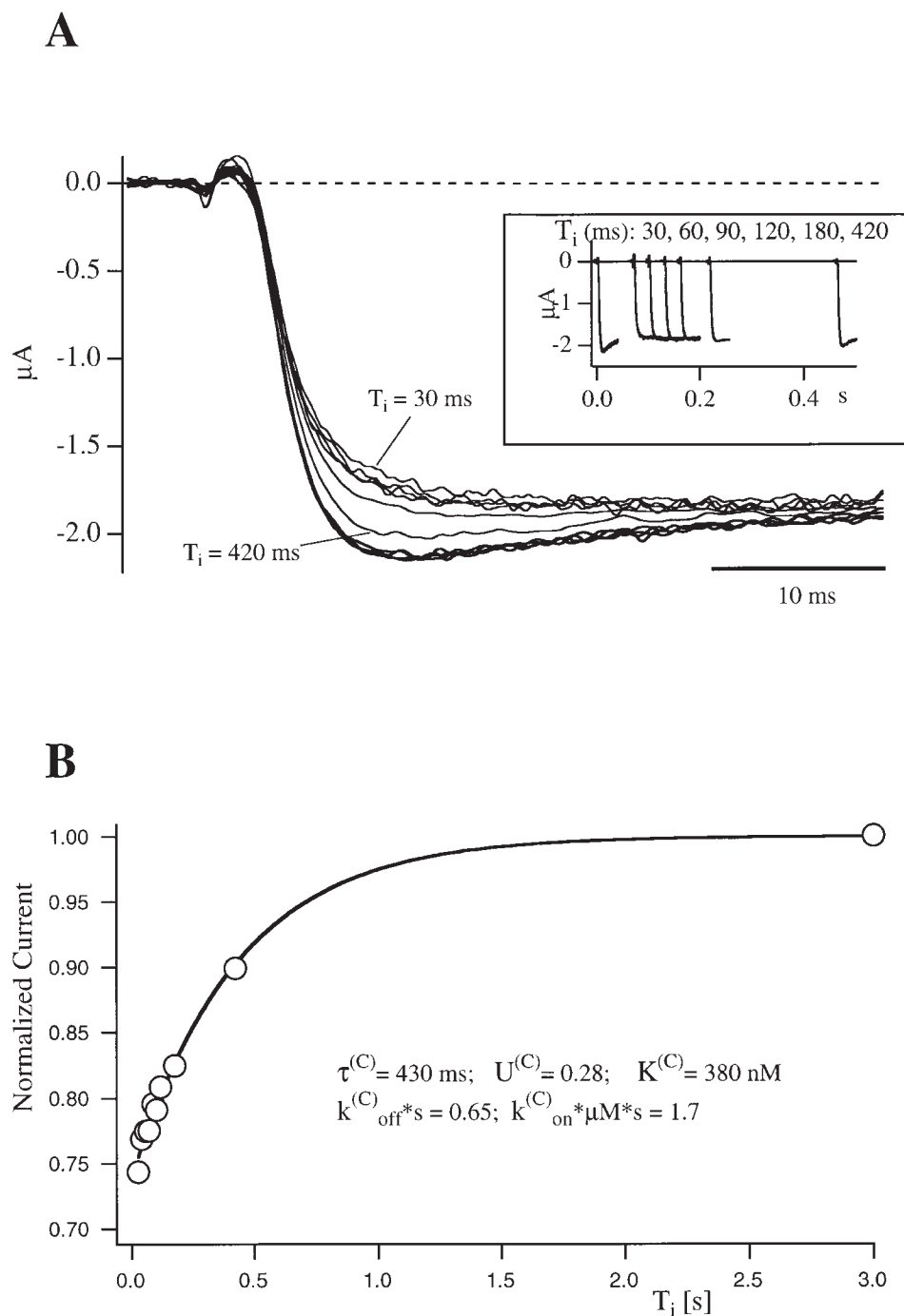
Figure 8. Recovery of tonic PVIIA binding to closed Sh \Delta channels in [K]_o = 115 mM. (A) Superimposed records of responses to double pulses of 40 ms at -20 mV with variable pulse interval, T_i ; the stimulation intervals at -100 mV were 3 s; the inset shows a sample of double responses in real time, whereas the main graph shows the same data with the second response translated to the time of onset of the first. The first pulse induces an increase of toxin block seen as a peak in the response; the peak reappears clearly in the second response only for T_i larger than hundreds of milliseconds. (B) The early amplitude of the second response is normalized to the first response and plotted as a function of T_i to follow the recovery of tonic block (the early amplitude was defined as the mean value of the current during the fixed interval in which the toxin free responses rise from 25 to 75% of their maximum); the solid line is the best fit with a single exponential with a time constant of 430 ms.
