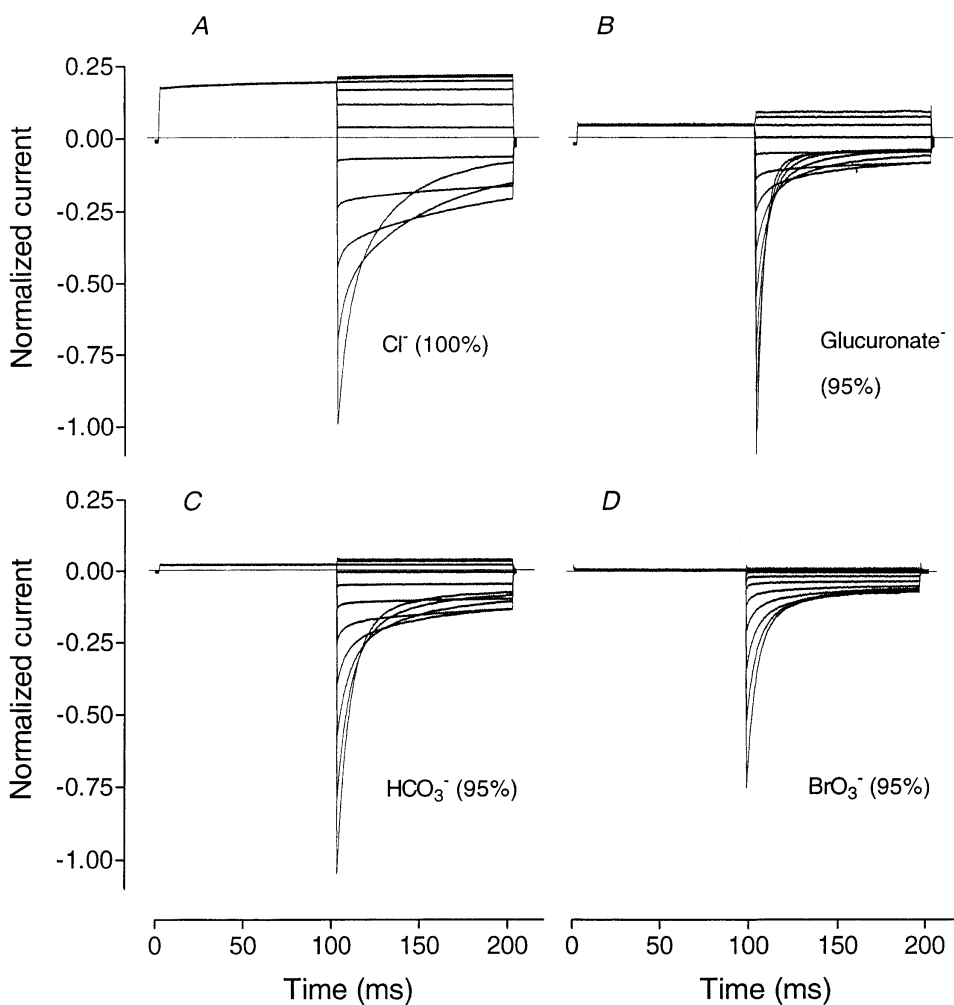
FIGURE 2. Kinetics of whole-cell currents in Sf9 cells expressing rClC-1 when impermeant or poorly permeant anions replace 95% of Cl - in the external solution. Currents were elicited by the standard activation protocol from a holding potential of -30 mV with a prepulse to +40 mV followed by steps from -120 to +80 mV in 20-mV increments. Since experiments were performed on different cells, currents have been normalized to the peak inward current in Cl - solution at -120 mV. Peak inward currents from cell to cell ranged between -5 and -10 nA.
