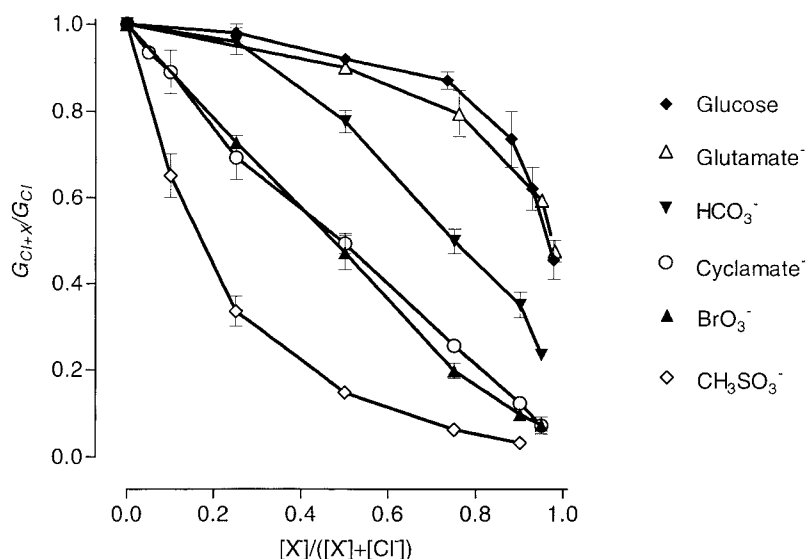
FIGURE 1. Membrane conductance of Sf9 cells expressing rClC-1 when impermeant or poorly permeant anions replace \text{Cl}^- in the external solution. Relative conductance, G_{X+Cl}/G_{Cl} , is plotted against mole fraction, [X^-]/([X^-]+[Cl^-]) , of the foreign anion. Conductance was estimated as explained in METHODS.
