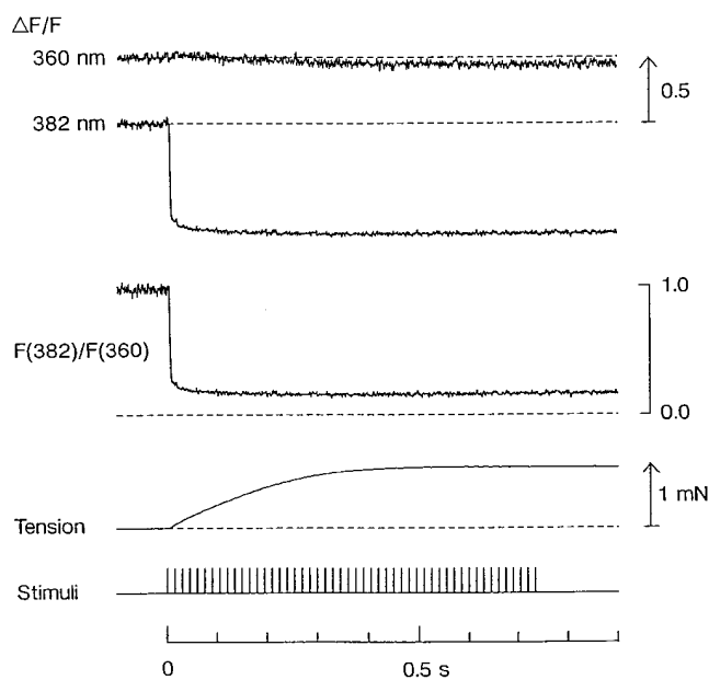
FIGURE 1. Fura dextran fluorescence and force records during high frequency stimulation in the presence of 10 μM TBQ. The muscle fiber was incubated in Ringer's solution containing 10 μM TBQ for 25 min. Fluorescence changes (ΔF) with excitation at 360 and 382 nm ( first and second traces) were normalized to the resting fluorescence level (F) at each wavelength, and are displayed as fractional changes (ΔF/F). The third trace is the fluorescence ratio R, and the fourth trace shows tetanic force. The bottom trace shows 50 stimuli (width 500 μs, interval 15 ms). Fiber, 112793f2; resting sarcomere length, 3.8 μm; indicator concentration, 91 μM.
