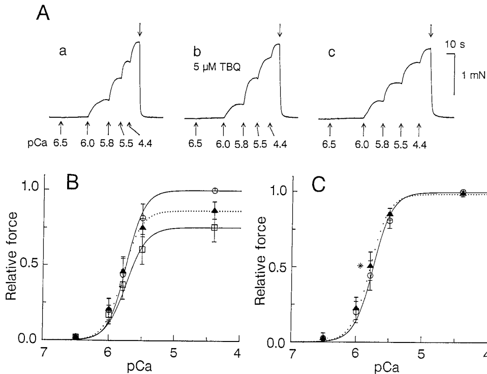
FIGURE 10. (A) Ca 2+ -activated force measurements in a skinned fiber repeated in the absence (a and c) and presence (b) of 5 μM TBQ. The records were taken in a sequence of a–c with 15-min intervals. In a–c, the bathing solution was changed sequentially from the relaxing solution to solutions of various [Ca 2+ ] i 's, as indicated in pCa units, and returned back to the relaxing solution (downward arrow). In b, 5 μM TBQ was applied for 2 min in the relaxing solution, and was maintained throughout the run. Fiber, 042795f4; resting sarcomere length, 2.8 μM. (B) Summary of [Ca 2+ ] i (pCa units)–force relation obtained as shown in A from six skinned fibers; symbols represent means ± SEM of data from the first run in the absence of TBQ (○), from the second run in the presence of 5 μM TBQ (▲), and from the third run after washout of TBQ (□). In each fiber, the steady force levels were
